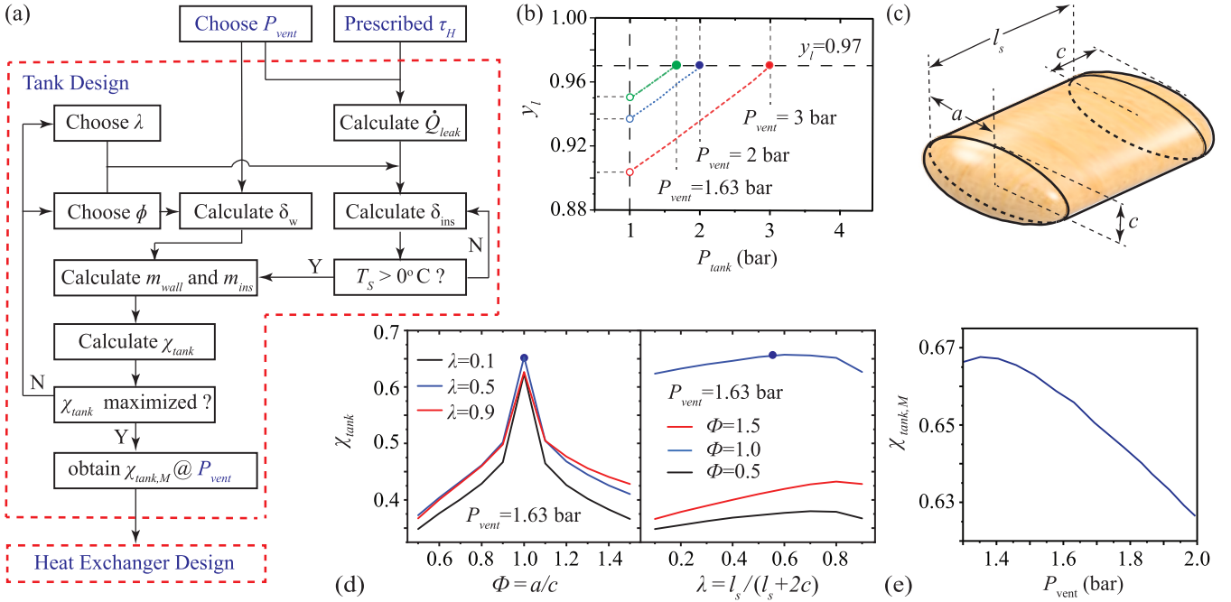
Fig. 3. (a) Flowchart showing the steps for LH 2 tank design. (b) Liquid volume fraction y_l in a closed LH 2 tank as a function of the tank pressure P_{tank} following initial filling at 1 bar. (c) Shape parameters a , c , l_s defining the tank geometry. (d) Variations of the tank gravimetric index \chi_{tank} with the tank's geometrical ratio parameters at P_{vent} = 1.63 bar. The maximum value \chi_{tank,M} is marked by the solid circles. (e) The obtained \chi_{tank,M} at different input parameter P_{vent} .
