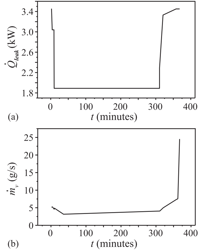
Fig. 7. (a) Calculated heat leakage rate \dot{Q}_{leak} through the hydrogen tank wall for the optimal design configuration; (b) derived vapor venting mass flow rate \dot{m}_v for maintaining the desired tank pressure profile during the flight.
