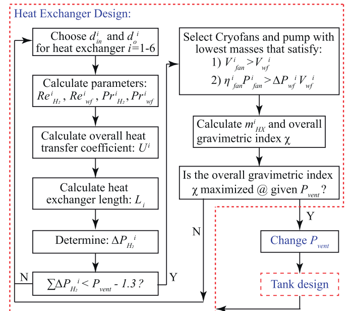
Fig. 4. Flowchart showing the steps for designing the heat exchangers.
