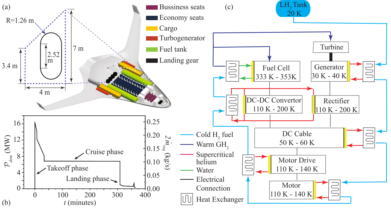
Fig. 1. (a) Layout of the blended wing-body airplane showing the space allocated for the liquid hydrogen fuel tank [14]. The inset displays the optimal tank geometry determined through the analysis presented in the text. (b) Flight power demand profile P_{dem}(t) for a short-range flight considered in our analysis. The corresponding required mass flow rate of hydrogen fuel 2\dot{m}_{req}(t) is also shown. (c) Schematic diagram illustrating hydrogen fuel flowing through heat exchangers associated with different power system components to provide cooling power before being fed into the fuel cell and combustion turboelectric generator.
