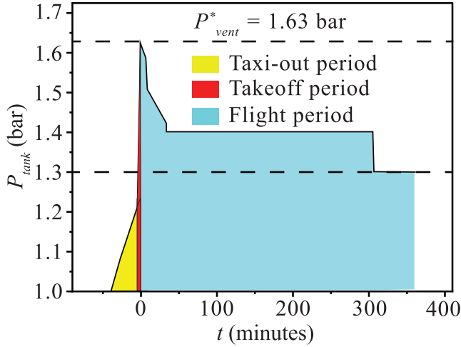
Fig. 6. Calculated tank pressure P_{tank} required to deliver fuel and meet the power demand shown in Fig. 1(a), using the optimal tank and heat exchanger configuration. A 40-min taxi-out period is included.
