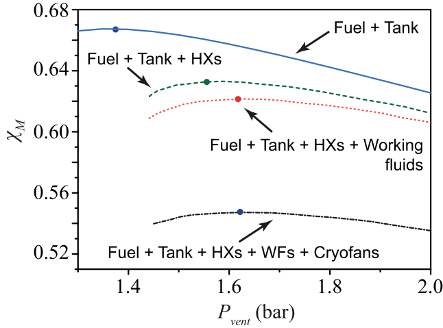
Fig. 5. Maximum overall gravimetric index, \chi_M , as a function of the design parameter P_{vent} . For comparison, \chi_M curves for analyses based on different contributions to the total mass are included.
