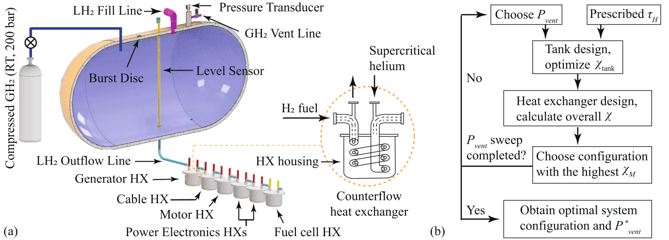
Fig. 2. (a) Schematic diagram showing the LH 2 storage tank (half-section), along with the heat exchangers through which hydrogen flows before reaching the fuel cells and the combustion turboelectric generators. The zoomed inset illustrates the counterflow heat exchanger for the generator. (b) Flowchart outlining the procedures for designing and optimizing the tank and thermal management systems.
